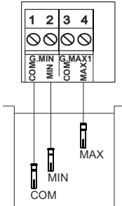
EXTERNAL COMMAND 2 INPUTS FILLING FUNCTION
